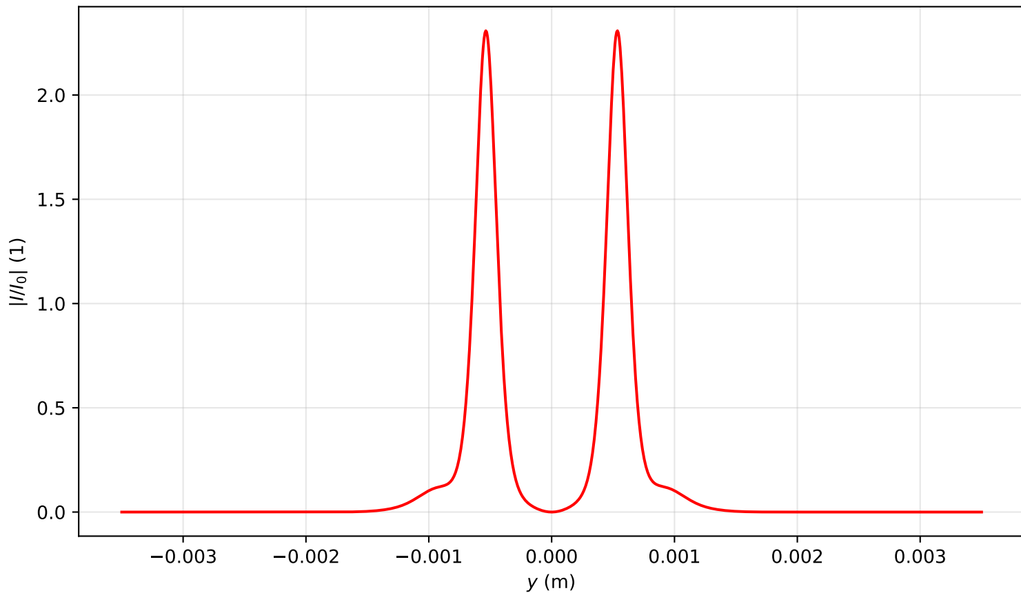
Intensity profile I(x=0, y, z=0.557)/I_0 , \text{Pin}=9.0\text{Pcr} , artificial time
